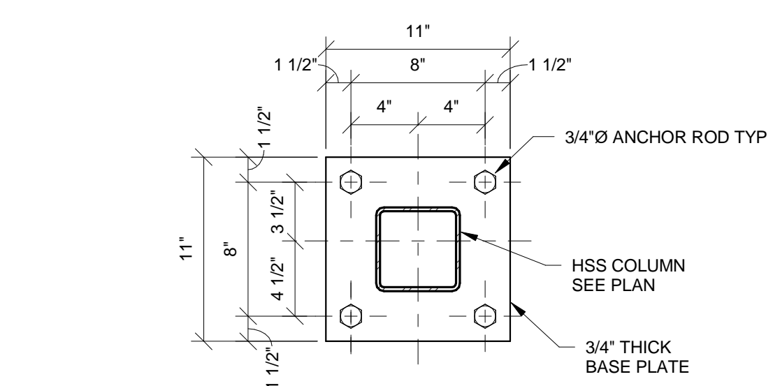
SECTION 17 SCALE 1 1/2" = 1'-0"
