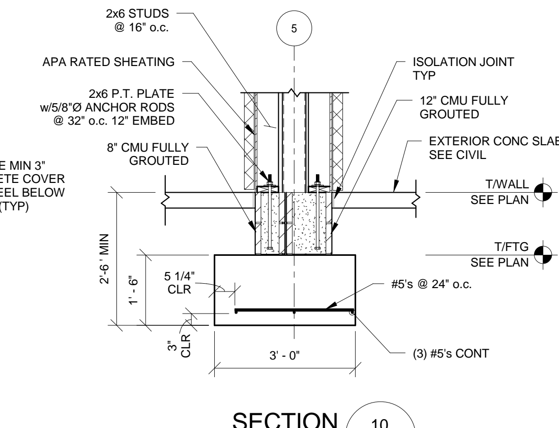
SECTION 10 SCALE 1/2" = 1'-0" S310
