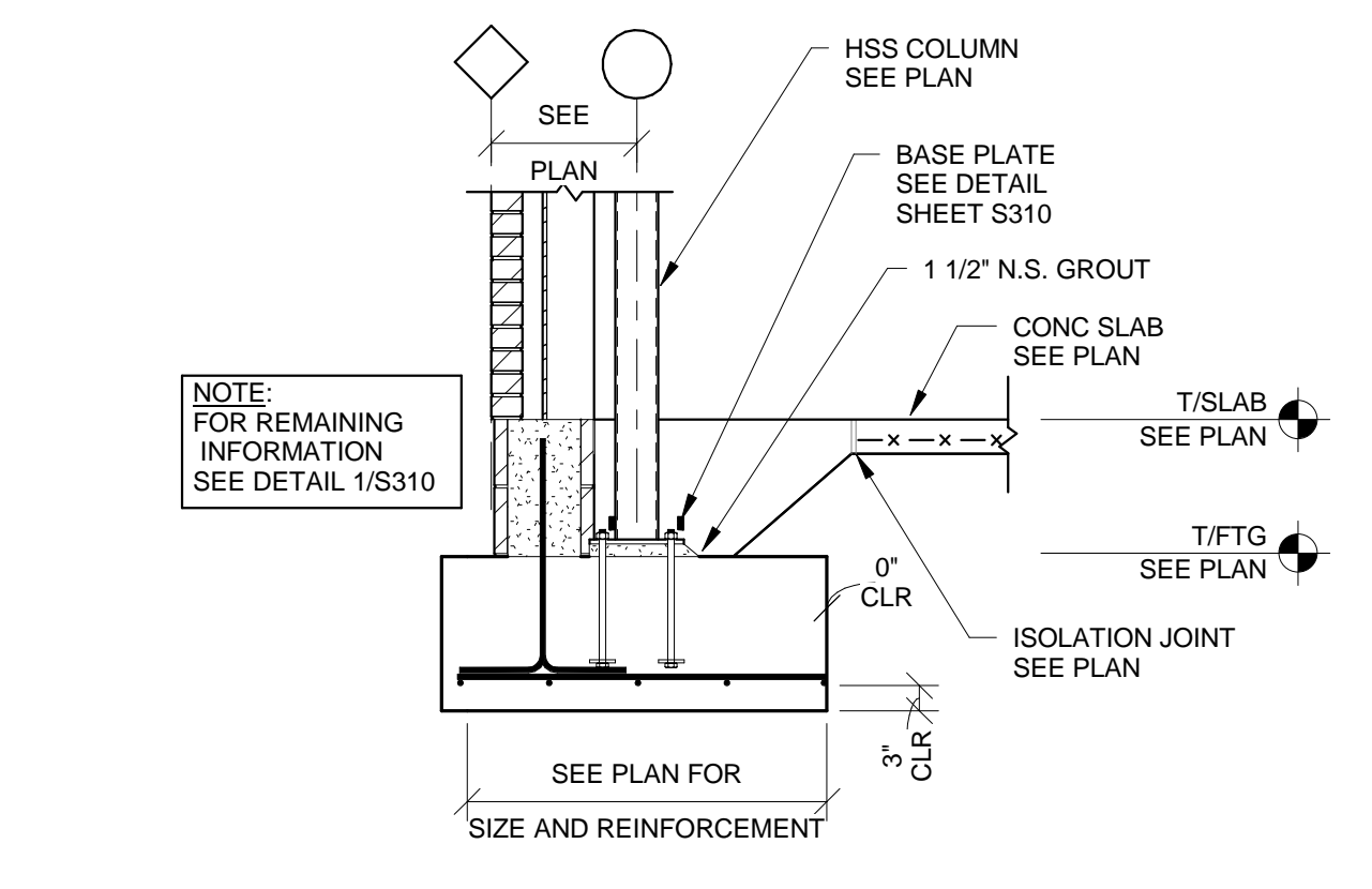
SECTION 5 SCALE 1/2" = 1'-0" S310
