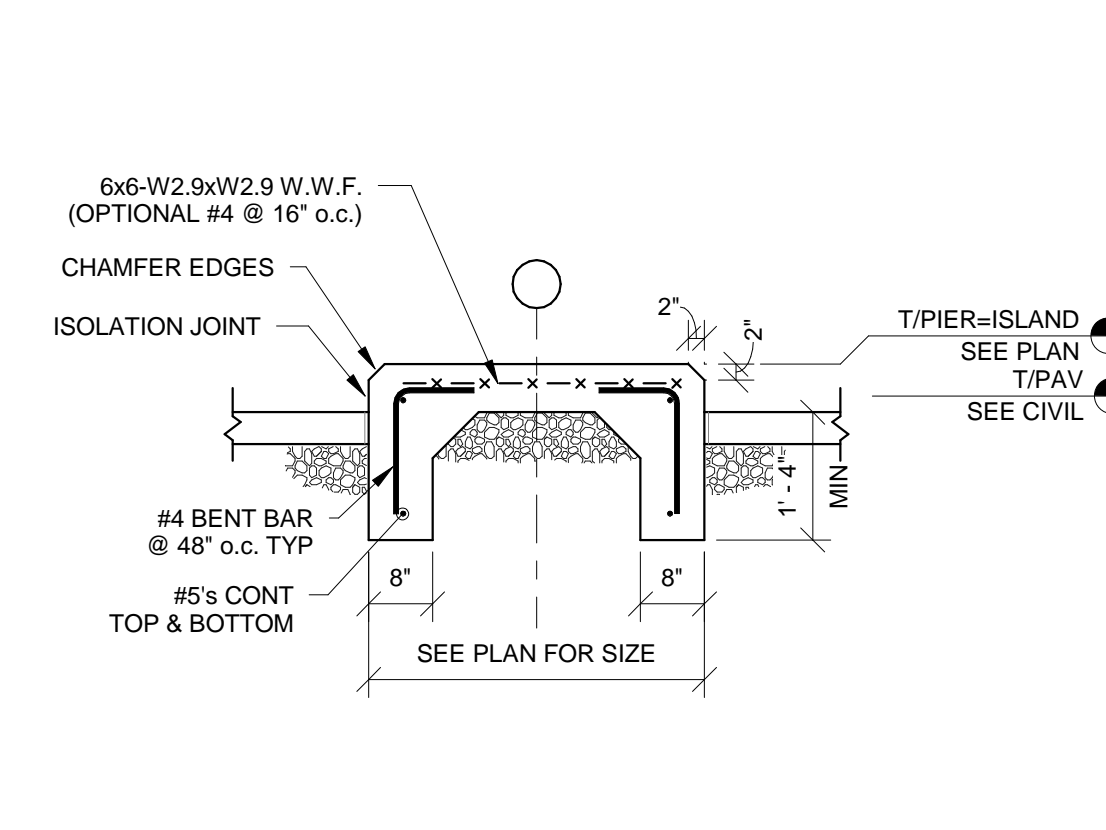
SECTION 7 SCALE 1/2" = 1'-0" S310
