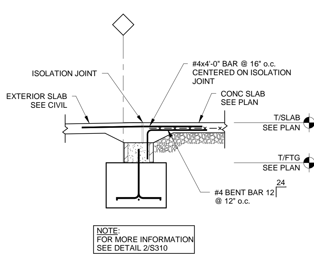
SECTION 3 SCALE 1/2" = 1'-0" S310
