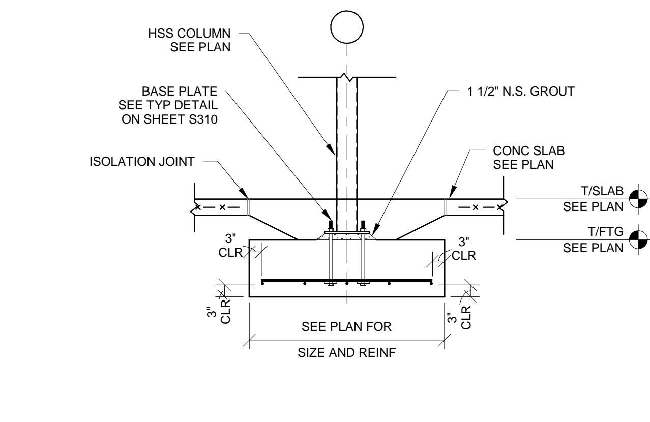
SECTION 4 SCALE 1/2" = 1'-0" S310
