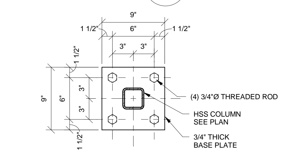
SECTION 11 SCALE 1 1/2" = 1'-0"
