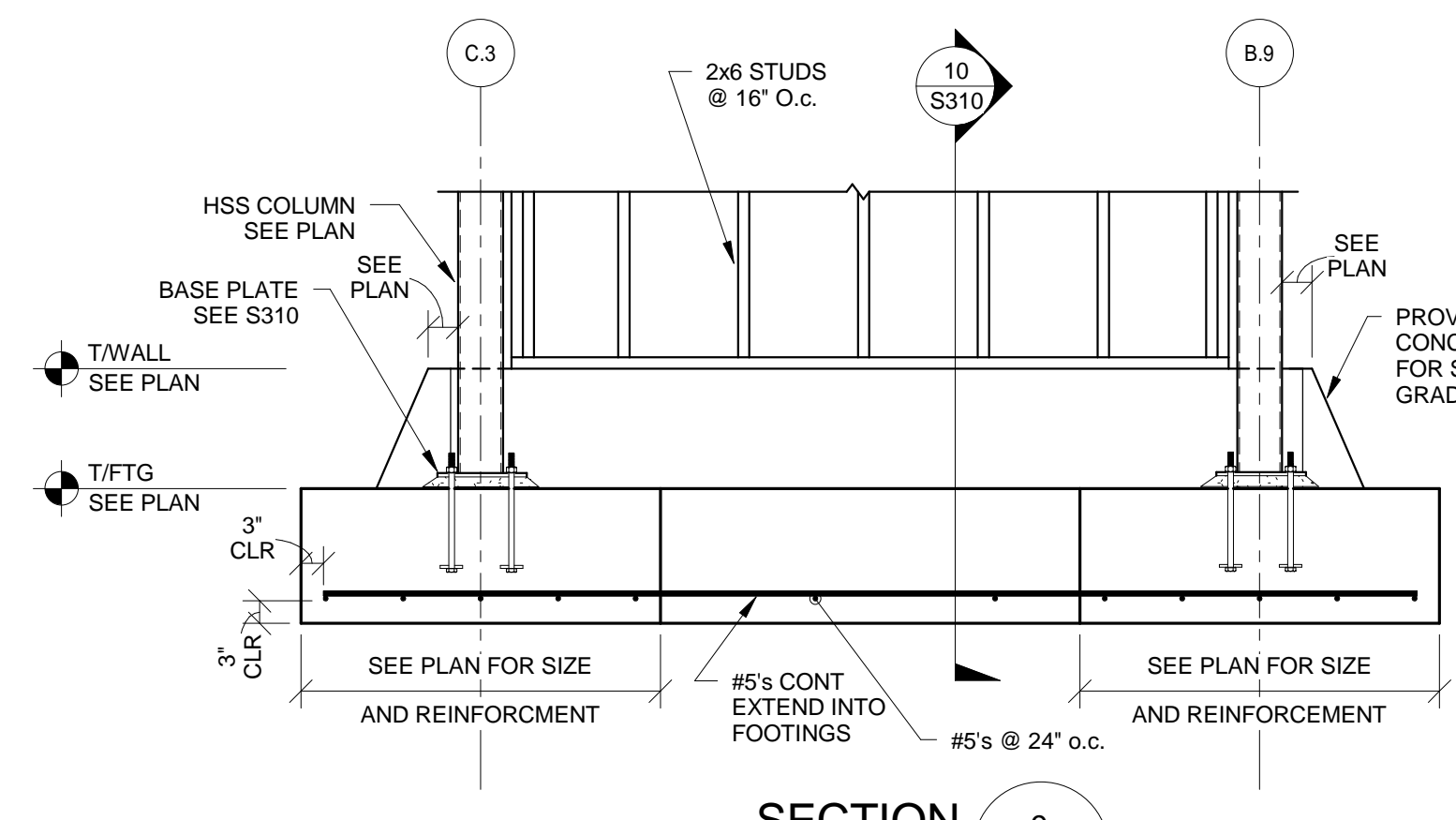
SECTION 9 SCALE 1/2" = 1'-0" S310
