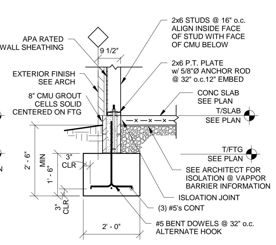
SECTION 2 SCALE 1/2" = 1'-0" S310
