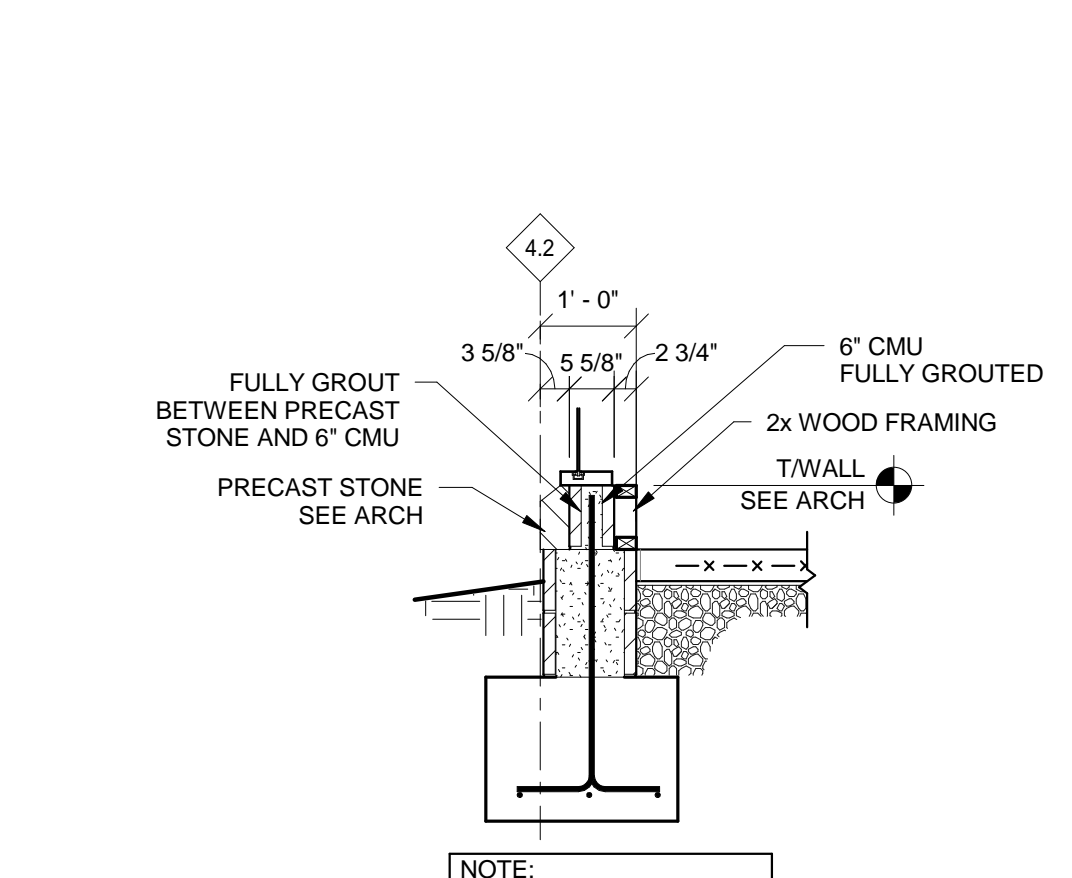
SECTION 9 SCALE 1/2" = 1'-0" S310
