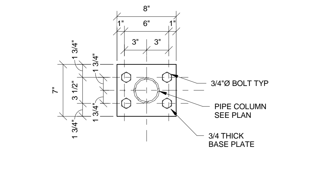
SECTION 16 SCALE 1 1/2" = 1'-0"
