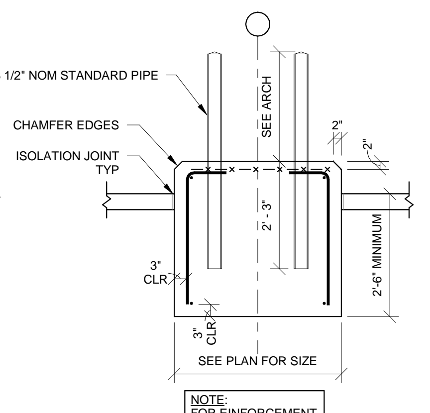
SECTION 8 SCALE 1/2" = 1'-0" S310
