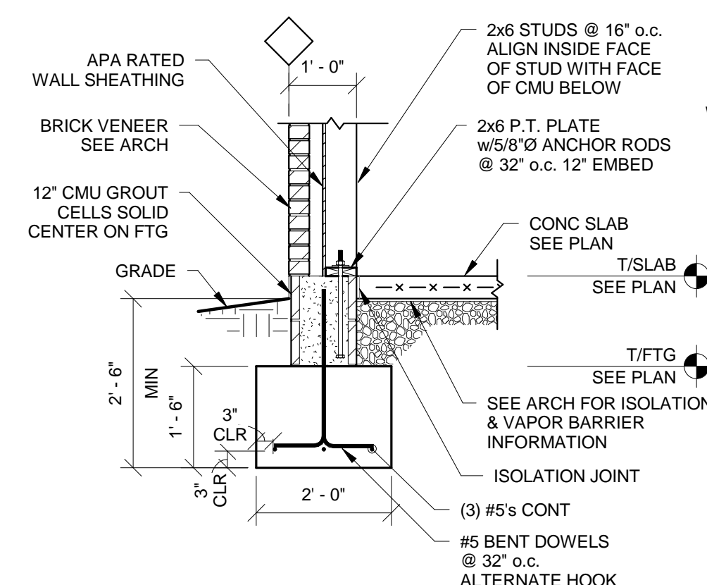
SECTION 1 SCALE 1/2" = 1'-0" S310
