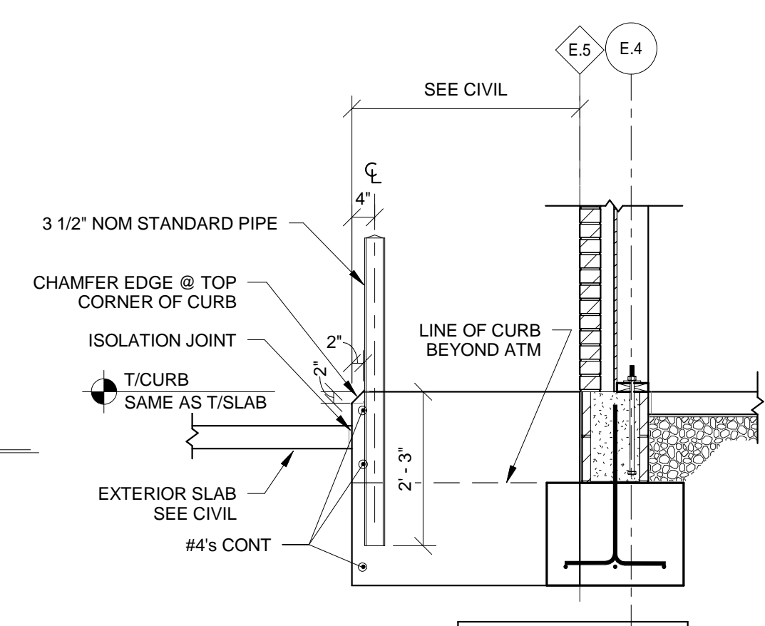
SECTION 8 SCALE 1/2" = 1'-0" S310
