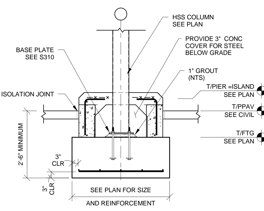
SECTION 6 SCALE 1/2" = 1'-0" S310
