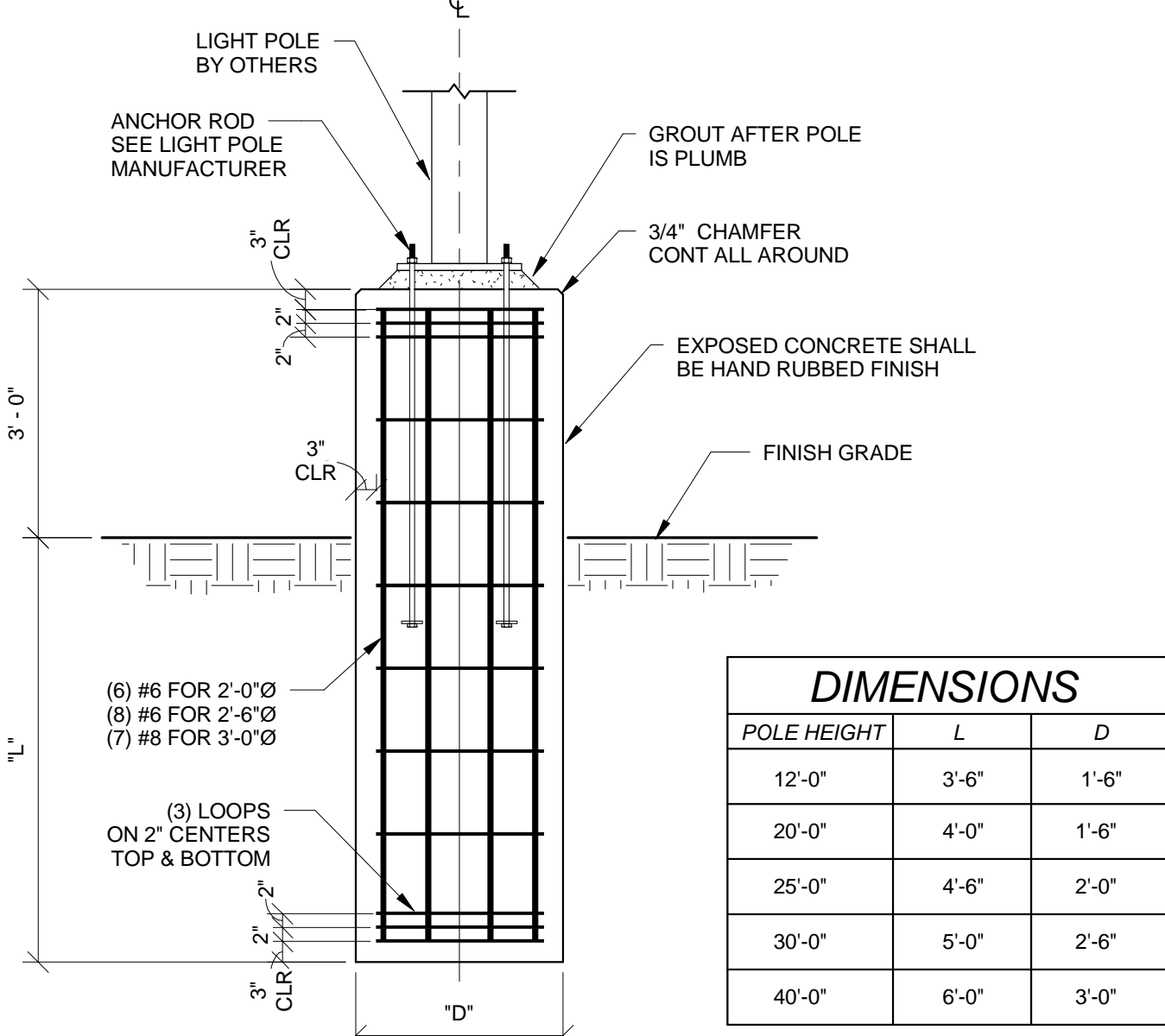
SECTION 20 SCALE 1/2" = 1'-0"
